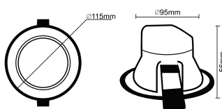
Dimension ( mm )
