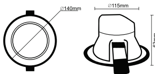
Dimension ( mm )
